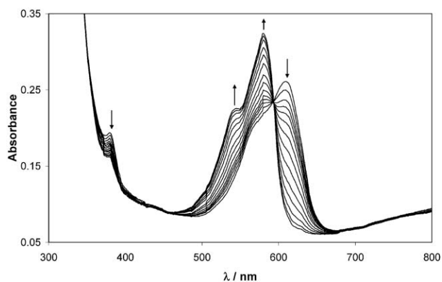
Fig. 2 UV/Visible absorption spectra of a sample of Activ TM (Pilkington Glass) coated with a film of the Rz/glycerol/HEC photocatalyst ink before and after UVA irradiation (using two 4 W BLB lamps; I = 12.4 \text{ mW cm}^{-2} ). The spectra were recorded every 30 seconds until no further significant changes occurred (after 6.5 mins). The dye initially present, resazurin, has an absorption peak at 610 nm and is reduced upon UV illumination, in the presence of a photocatalyst, to resorufin, which absorbs at 585 nm. Note: if coated on plain glass, the ink has the same spectrum as that shown for t = 0 ( i.e. spectrum where absorbance at 610 nm is a maximum), and does not change even after prolonged UVA irradiation ( i.e. >1 h).
